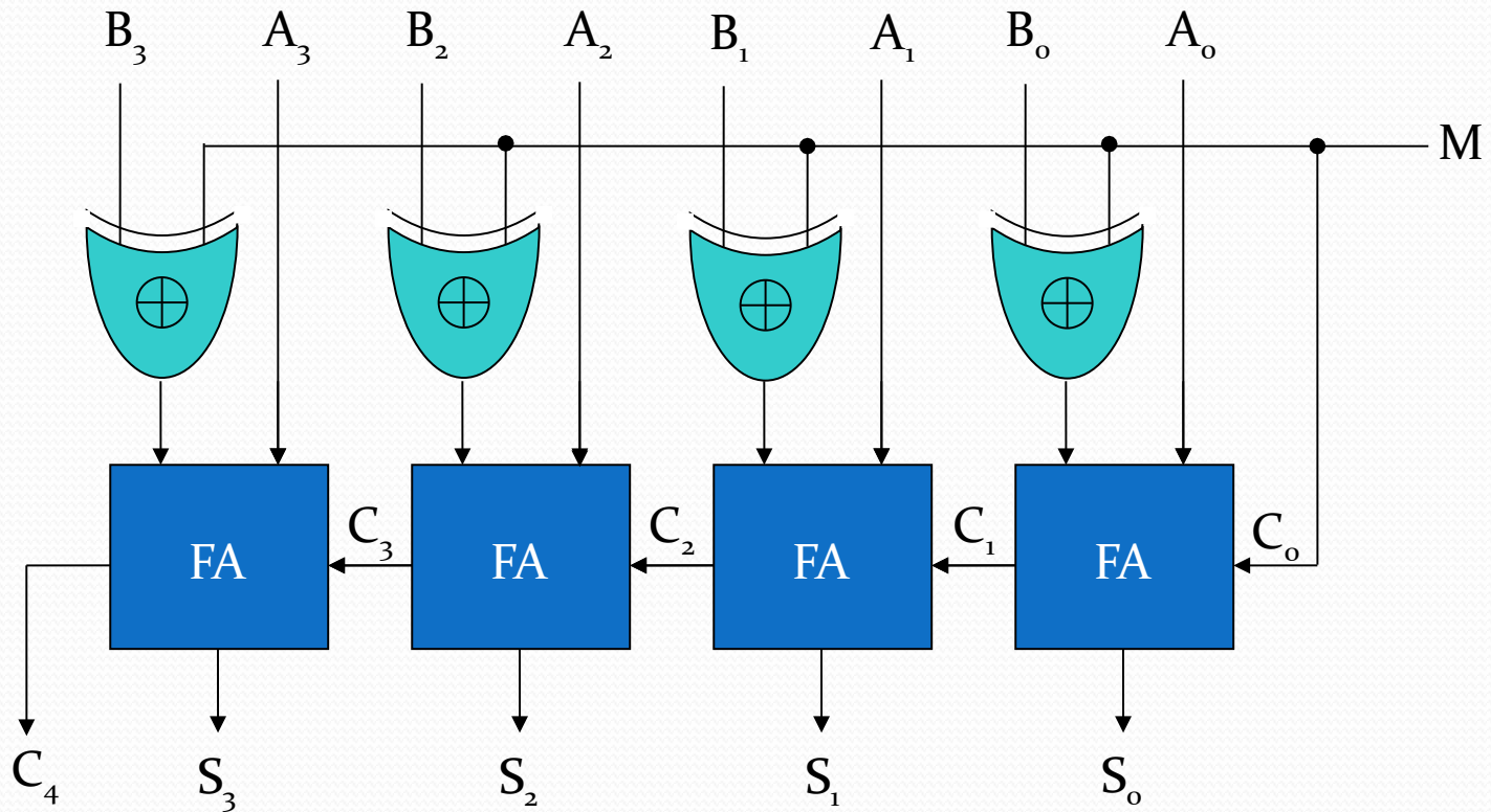
4-bit adder-subtractor
